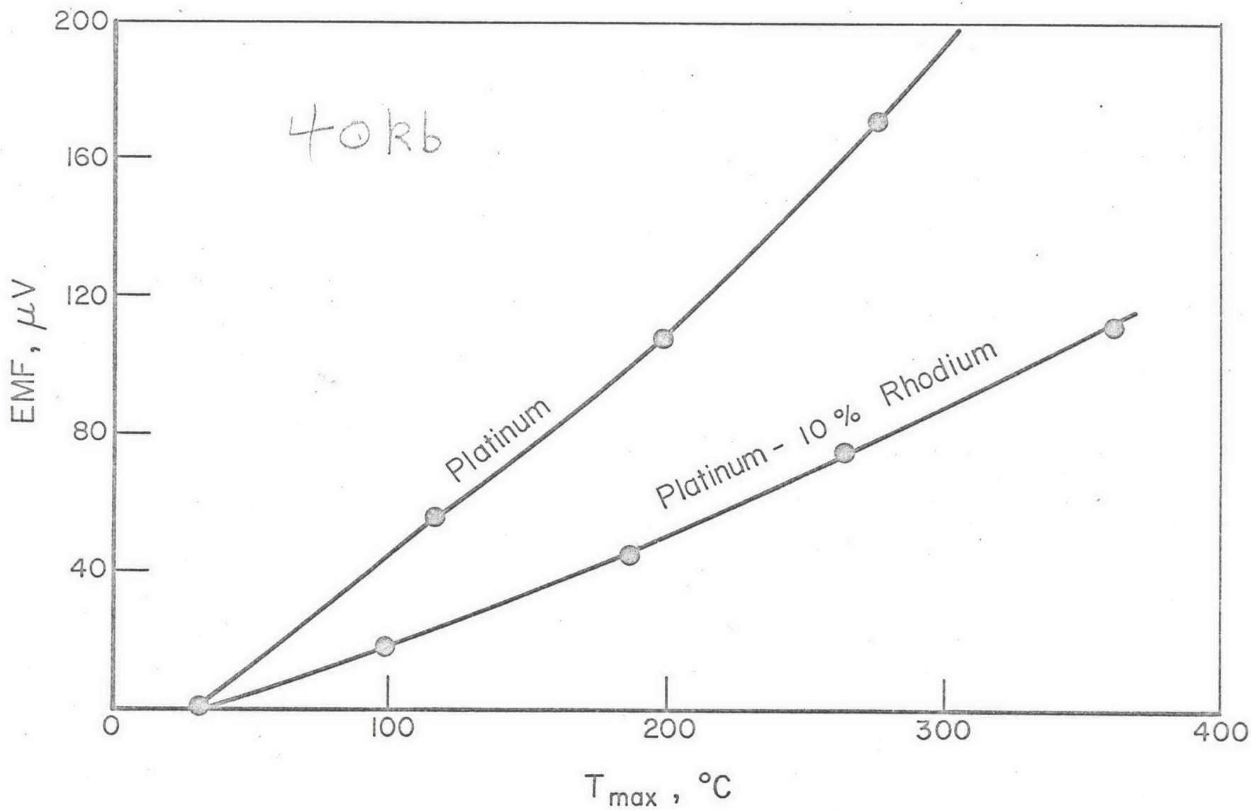
PRESSURE EMF VERSUS TEMPERATURE PLATINUM-PLATINUM 10% RHODIUM
